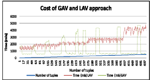
Figure9. Cost of GAV and LAV approach
