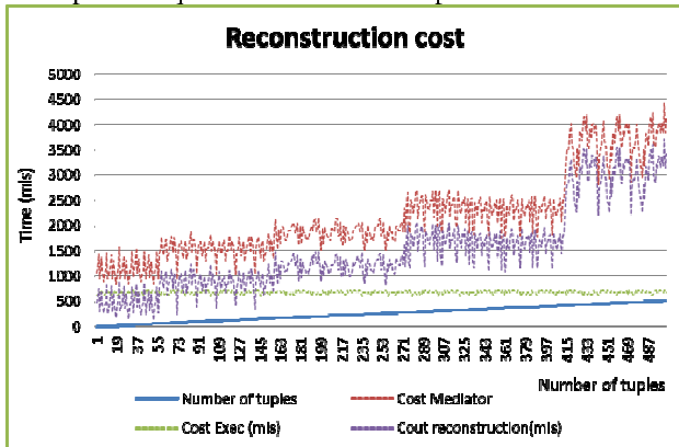
Figure8. Cost of reconstruction
