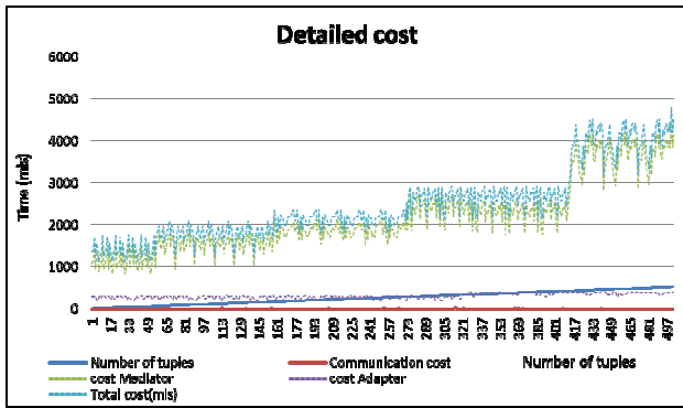
Figure7. Time of each phase
