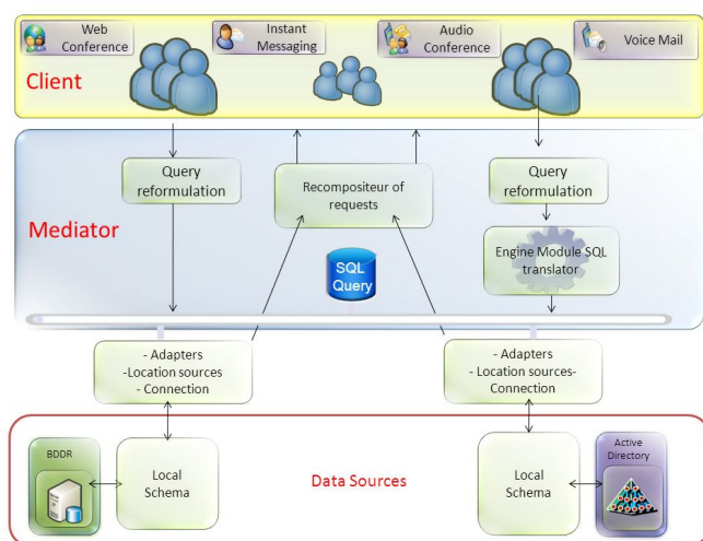
Figure2. Architecture of the prototype mediation.
