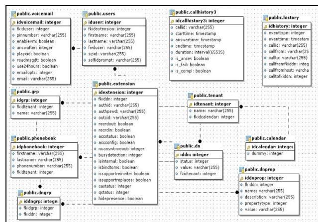
Figure3. Diagram of the database 3CX.
