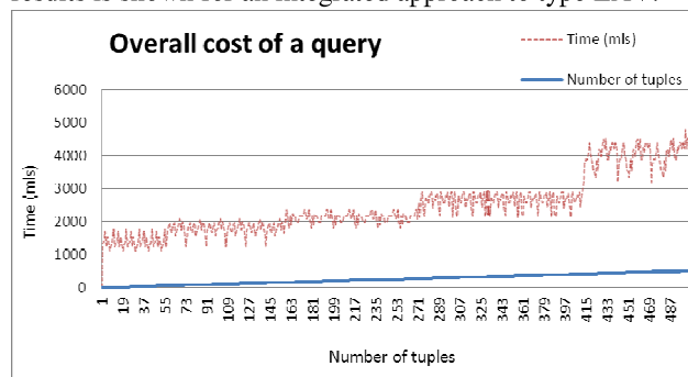
Figure6. Cost of a query
