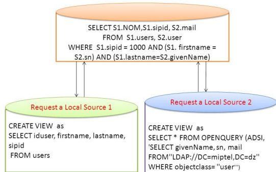
Figure4. Decomposition of the global query
